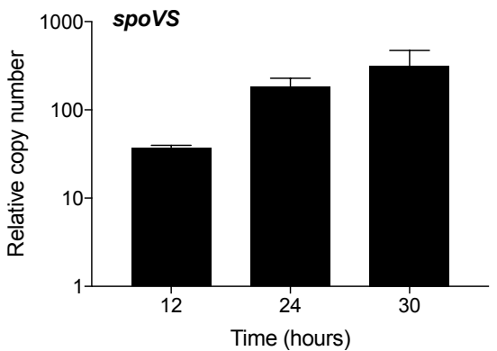
Figure S3. Quantitative reverse transcriptase PCR of six genes identified as differentially expressed in the RNA Seq analysis. Expression was quantified via standard curve and was normalized to the expression of rpoC . Information on primers can be found in Table S1.
