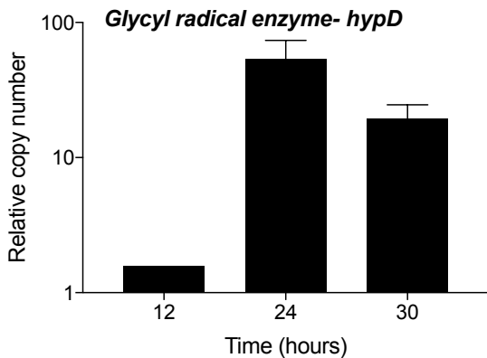
Figure S3. Quantitative reverse transcriptase PCR of six genes identified as differentially expressed in the RNA Seq analysis. Expression was quantified via standard curve and was normalized to the expression of rpoC . Information on primers can be found in Table S1.
