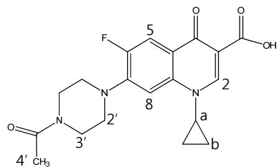
N-Acetylciprofloxacin
